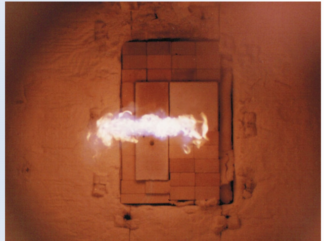
QVW003G000 at 2 MMBtu/hr Adjustment for Level Firing
