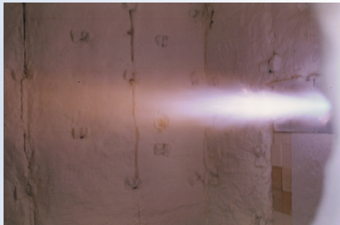
QS001G000 at 1 MMBtu/hr High Momemtum Setting
