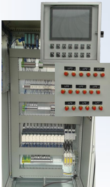
MULTIPLE MOTOR STARTER BAGHOUSE CONTROL WITH PLC/HMI, LOCAL I/O AND DIFFERENTIAL PRESSURE TRANSMITTERS
