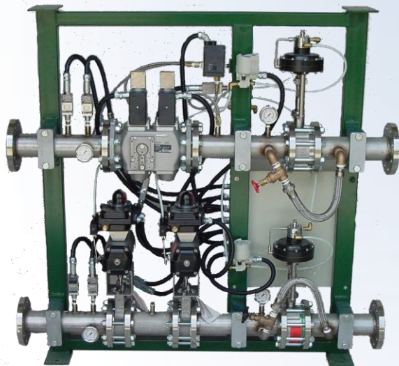
NATURAL GAS/OXYGEN FLOW CONTROL & SAFETY SHUT-OFF W/LOCAL SHUT-OFF W/INTEGRATED PLC/IO DROP
