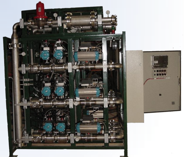
THREE ZONE OXYGEN/NATURAL GAS SAFETY SHUT-OFF W/PRESSURE REGULATION/FILTRATION FLOW CONTROL & MEASURE W/PLC/IO DROP
